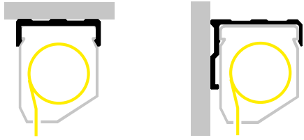
Cass. 64mm a soffitto Box 64mm Top fixing
