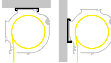
Cass.80mm a soffitto Box 80mm Top fixing
